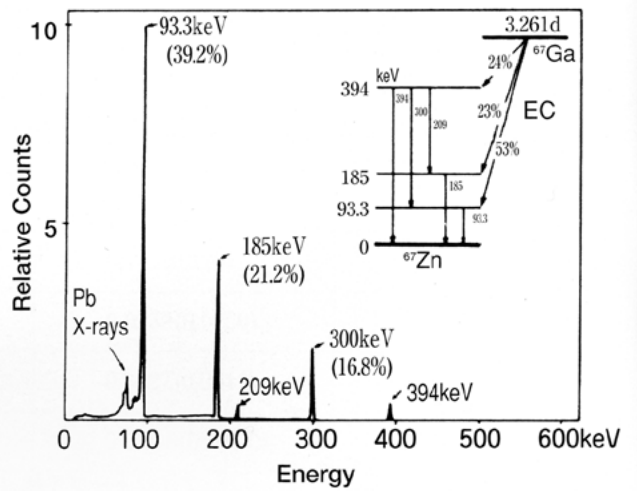
Ga-67
